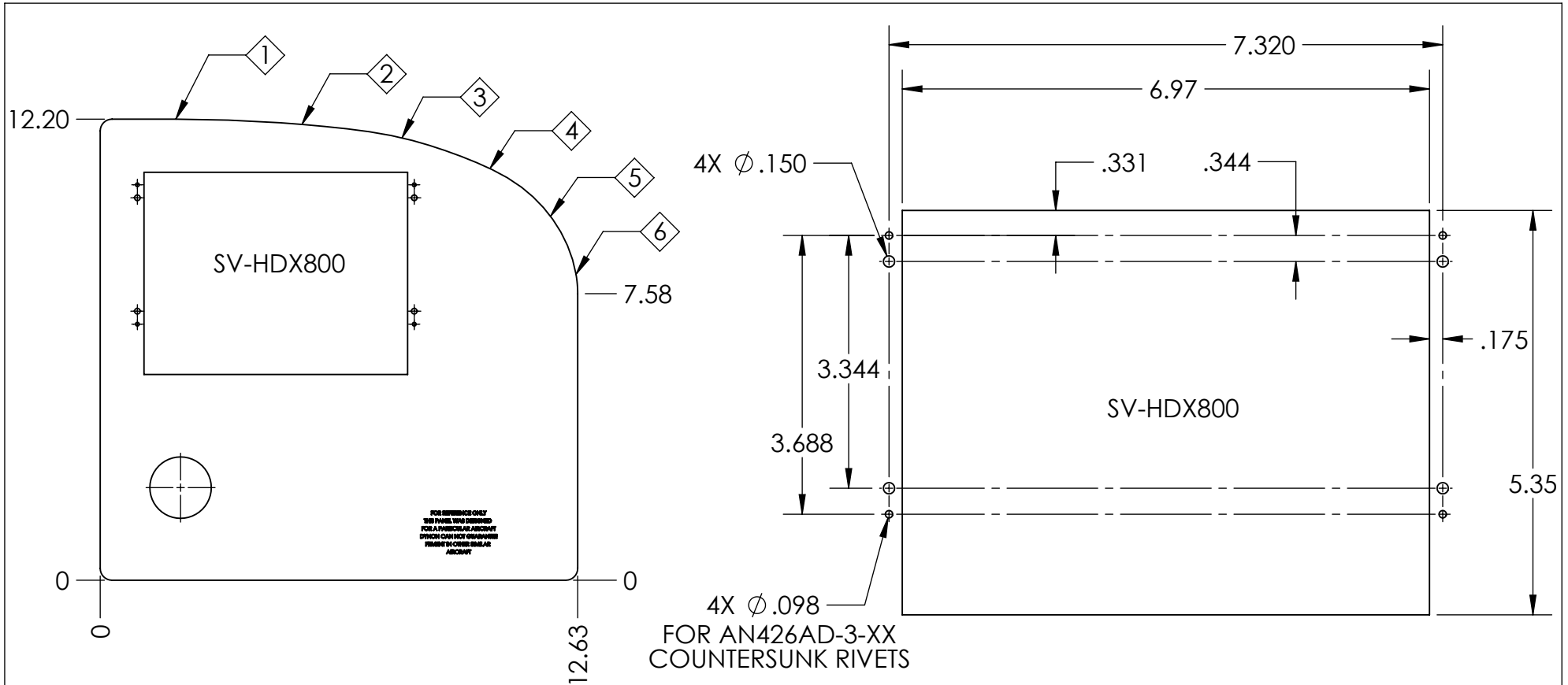
DETAIL B SCALE 1 : 2
