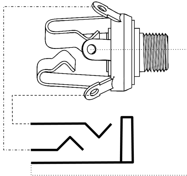
Figure 9: Headset Jack Schematic Symbol Guide
