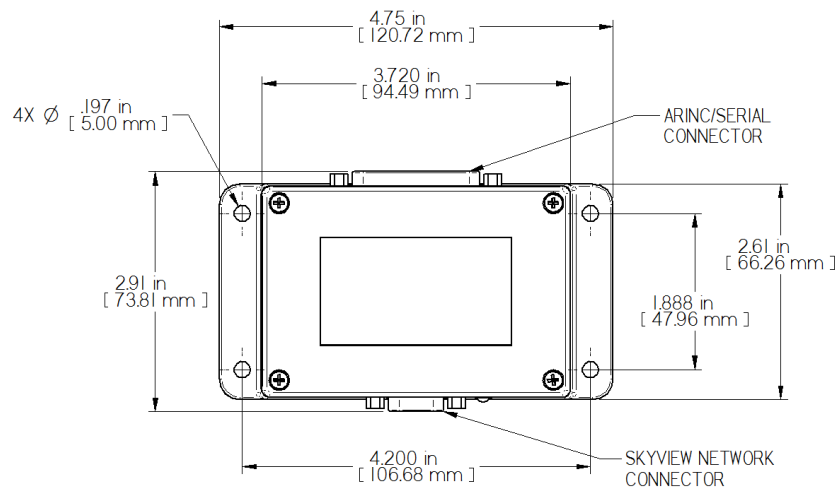
Figure — SV-ARINC-429 Mounting Dimensions with Electrical Connections
