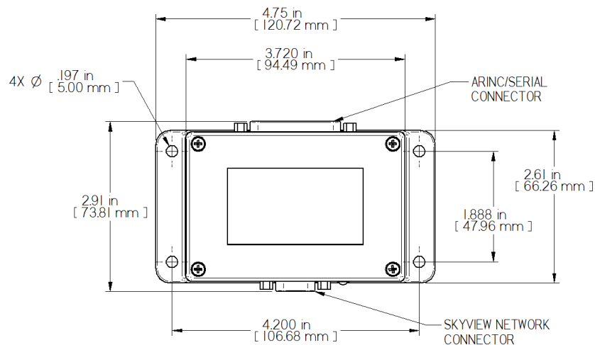
Figure 177 – SV-ARINC-429 Mounting Dimensions with Electrical Connections
